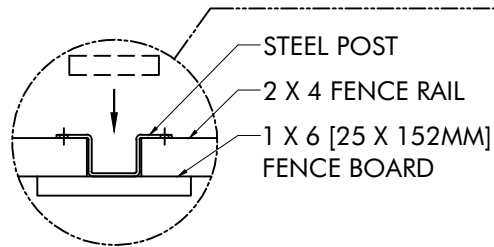
PLAN DETAIL (4X SCALE)
